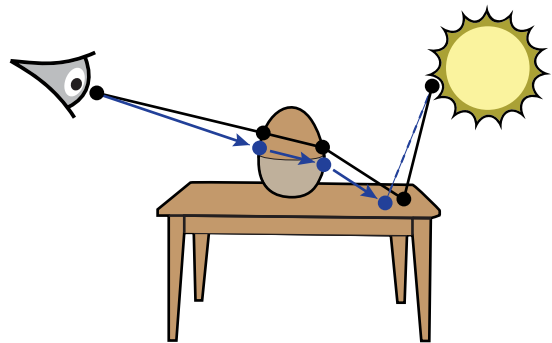
(a) Lens perturbation
