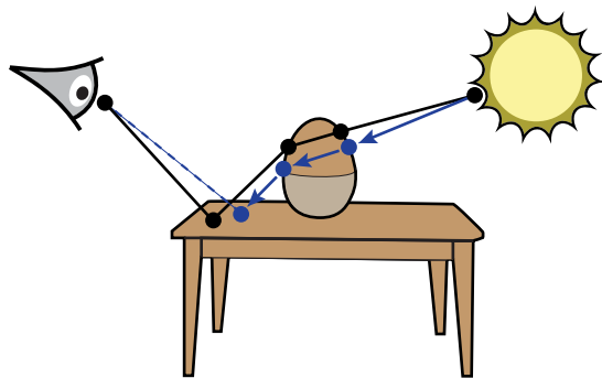
(b) Caustic perturbation
