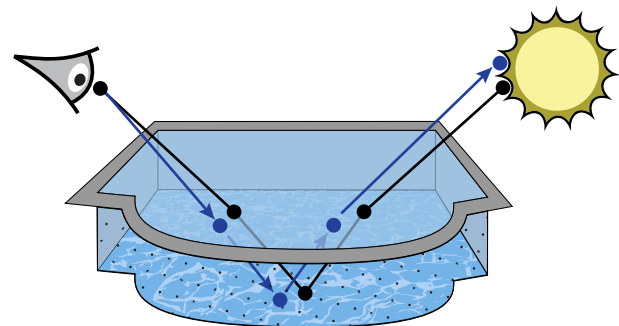
(c) Multi-chain perturbation
